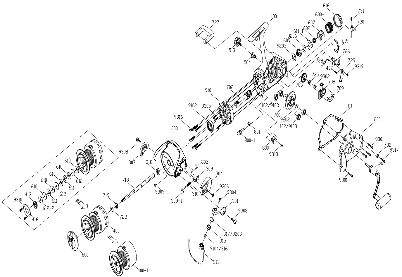
ABF - 90 Spare Parts
